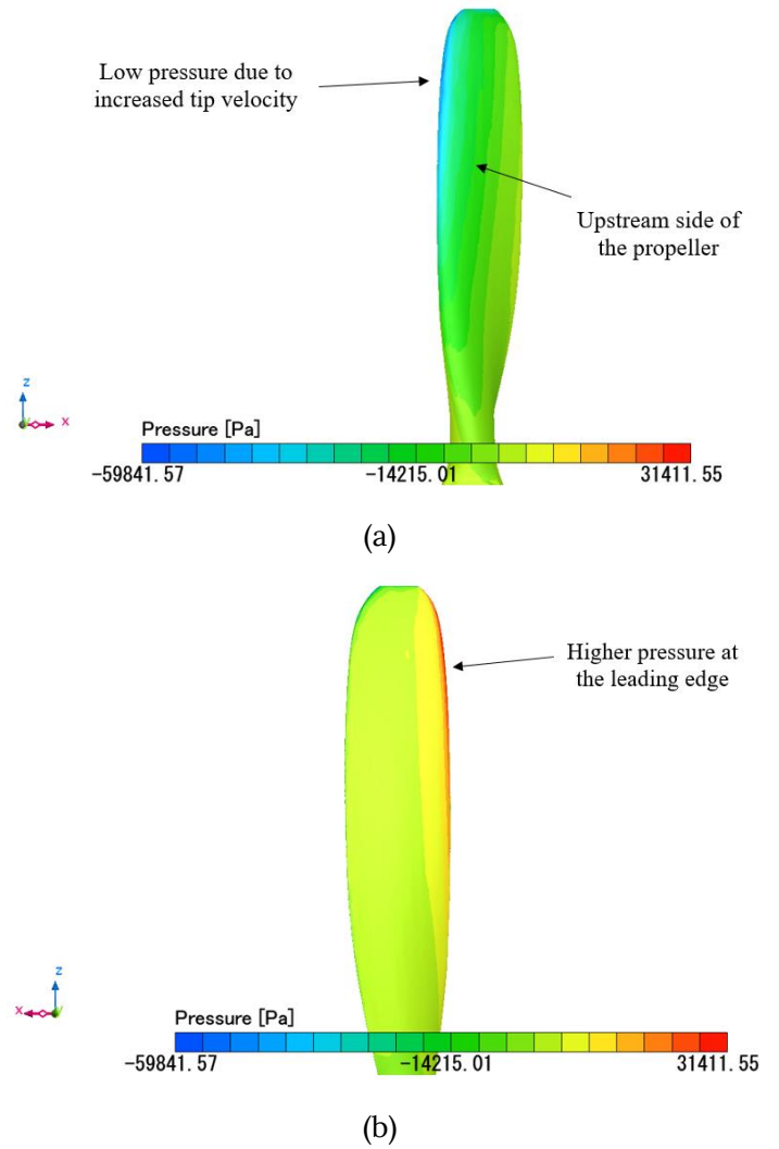
Fig. 10. Pressure distribution over the propeller: (a) pressure contours on the upstream side of the propeller (3100RPM) and (b) pressure contours on the downstream side of the propeller (3100RPM)
